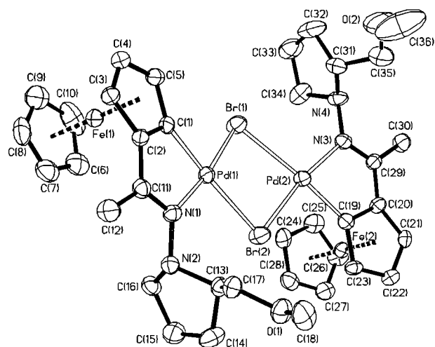
Fig. 3 Molecular structure (30% thermal ellipsoids) and absolute configuration of complex syn -(+)-(R p ,R,R,R p )-5 with atom-numbering scheme.
